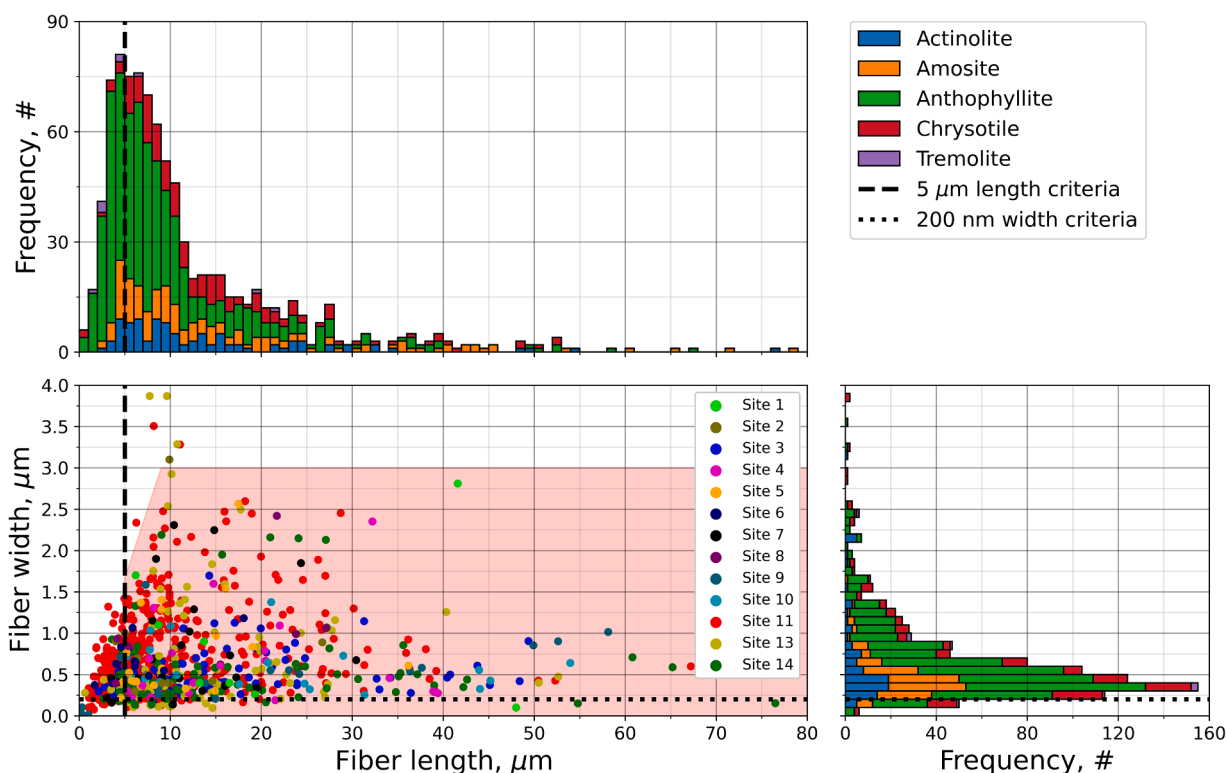
Fig. 4. Top: Histogram of asbestos fiber lengths in 1 \mu\text{m} bins colored according to asbestos type. The 5 \mu\text{m} WHO length criteria is marked as a dashed line. Bottom left: Scatter plot of asbestos fiber lengths and widths colored according to site. Red area marks dimensions fulfilling WHO fiber criteria. Bottom right: Histogram of asbestos fiber widths in 100 nm bins colored according to asbestos type. Estimated resolution limit of 200 nm is marked by dotted line.
