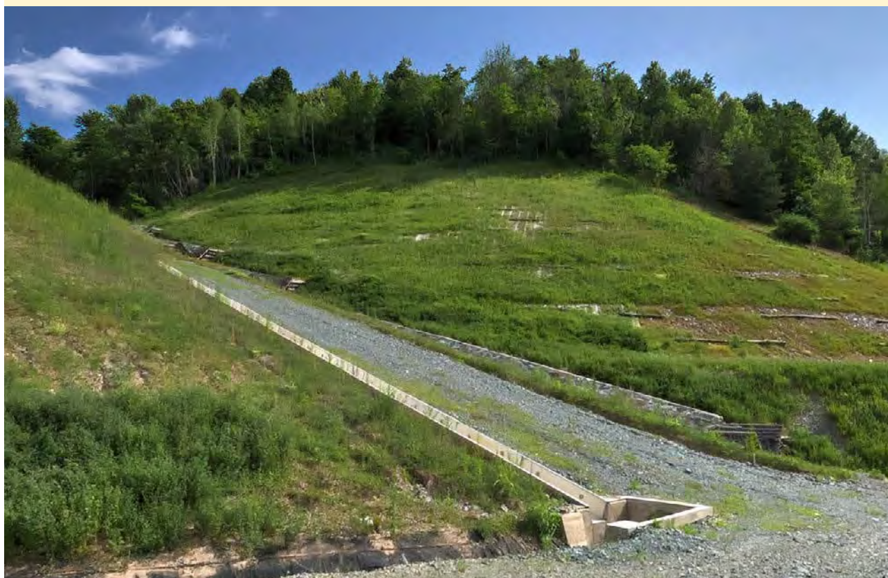
Figure 15-10: Area A after remediation: stabilised slopes covered in vegetation prevent the release of airborne dust
